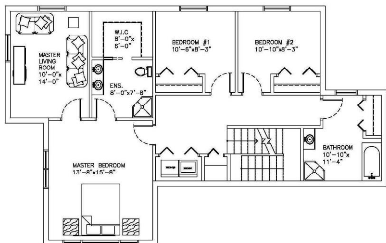
Second floor plan 1060 Sq.Ft
