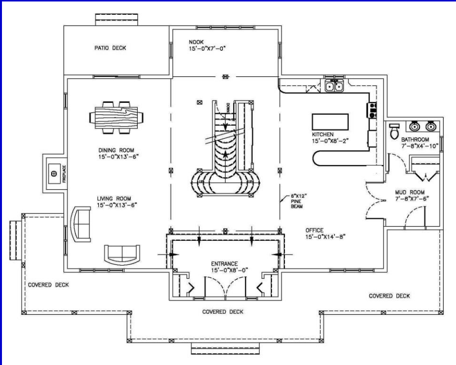
Main floor plan 1500 Sq.Ft
