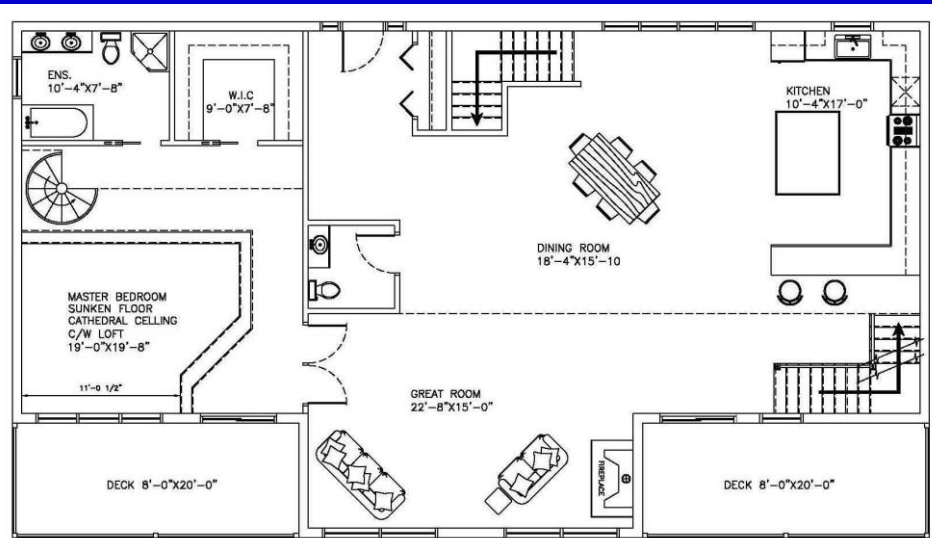
Main floor plan 1852 Sq.Ft
