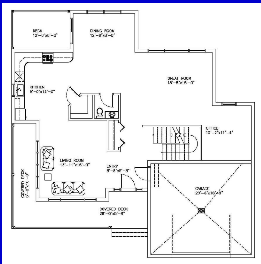
Main floor plan 1211 Sq.Ft
